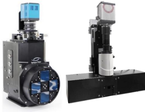
Zoom White Beam 4 scintillators
