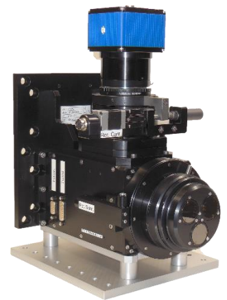
Monochromatic 3 objectives / 3 scintillators
