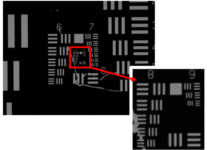
Highest frequency: Group 9 / Element 3 645.1 Line pairs per mm ; line width = 0.78 μm
